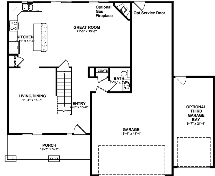
MAIN LEVEL FLOOR PLAN 819 sq ft
