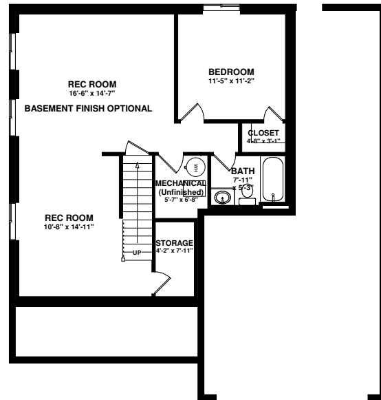
BASEMENT FLOOR PLAN 863 sq ft
